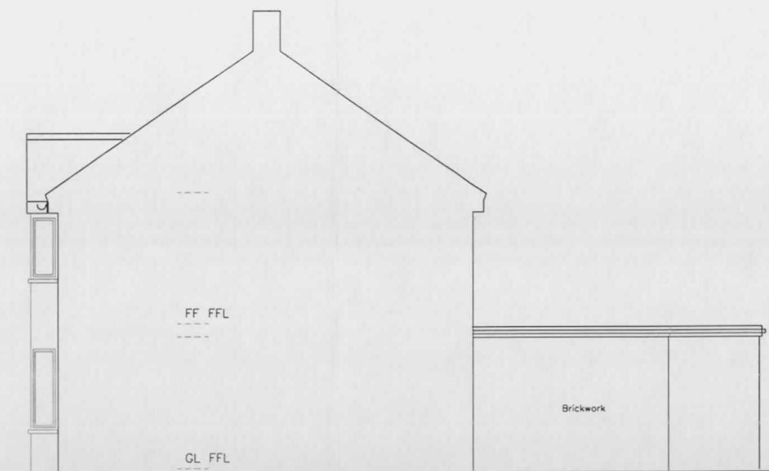
Side Elevation 1:100
