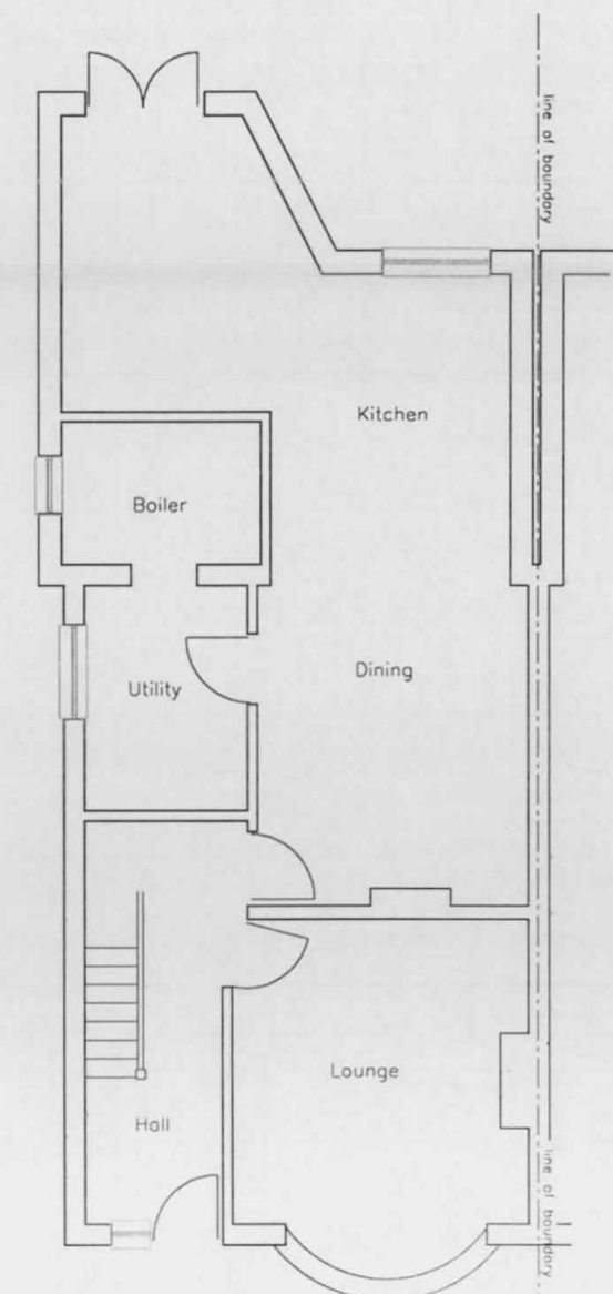
Ground floor plan 1:100
