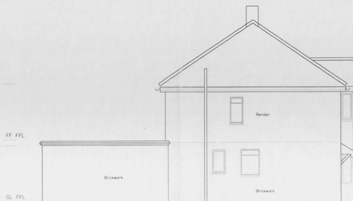
Side Elevation 1:100
