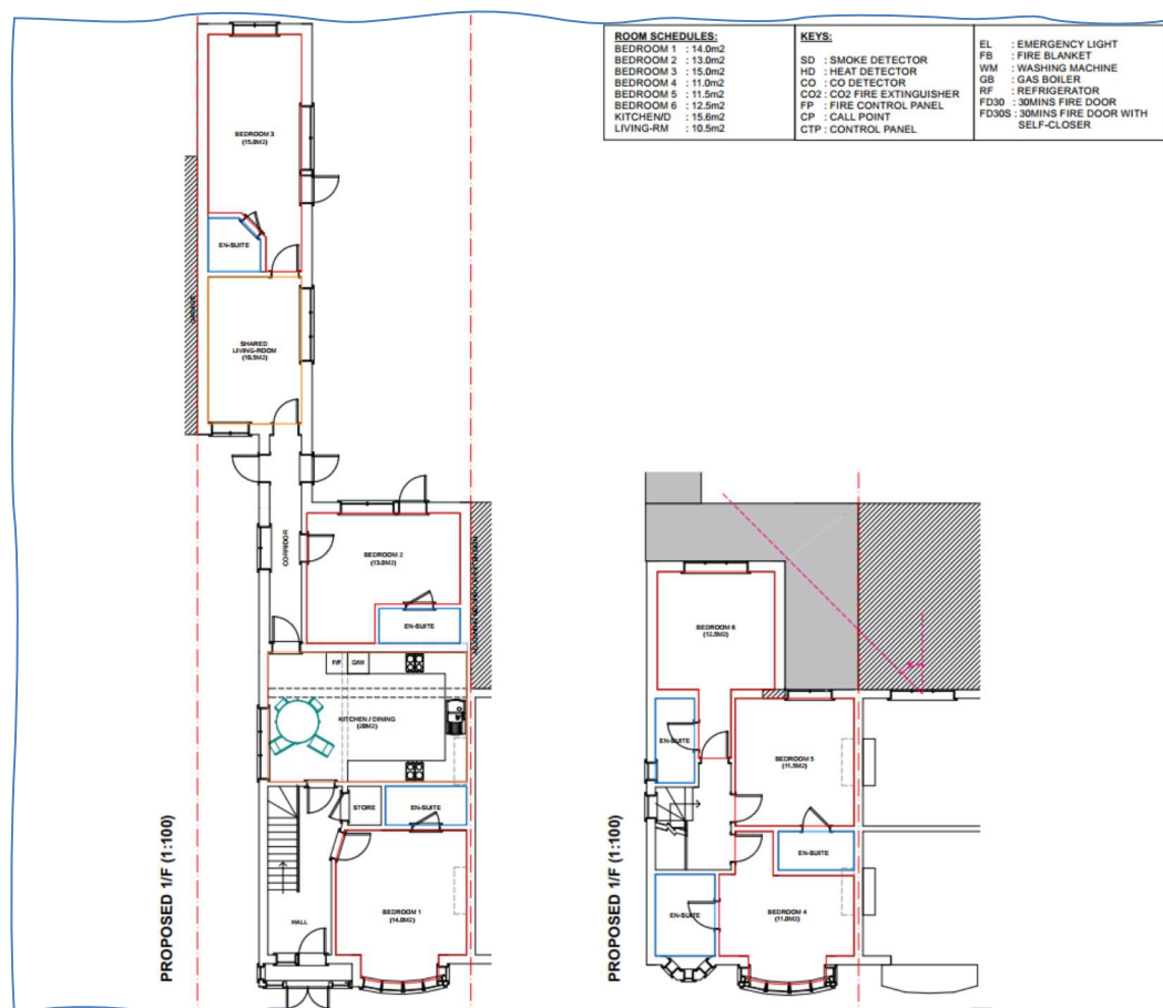
Fig. 2: The proposed C4 HMO floor plan
