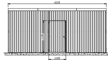
BIKE STORE 1:50
