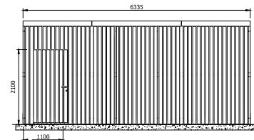
BIN STORE 1:50
