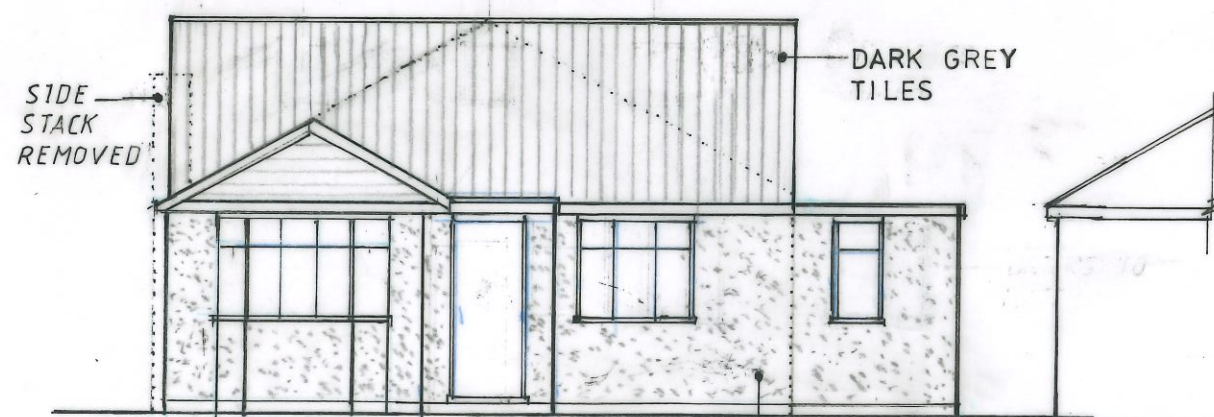
PROPOSED FRONT
