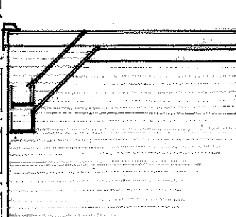
BOX GUTTER DETAIL
