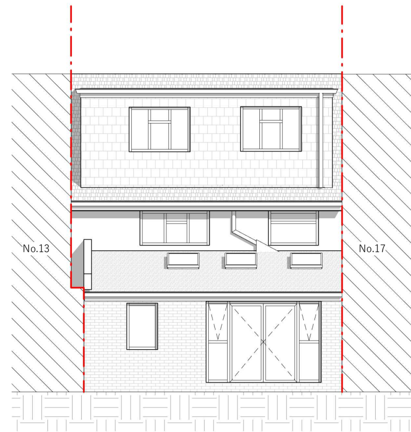
3 Proposed Rear Elevation 1 : 100
