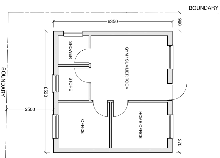
FLOOR PLAN
