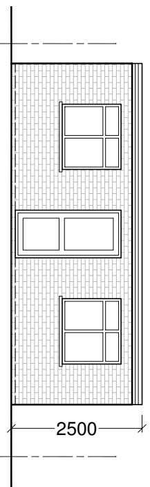
NORTH ELEVATION
