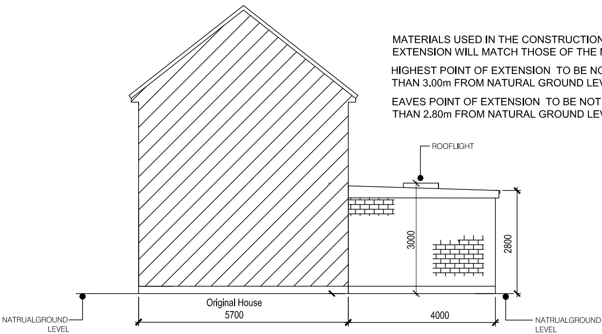
PROPOSED-SIDE ELEVATION (RHSIDE)
