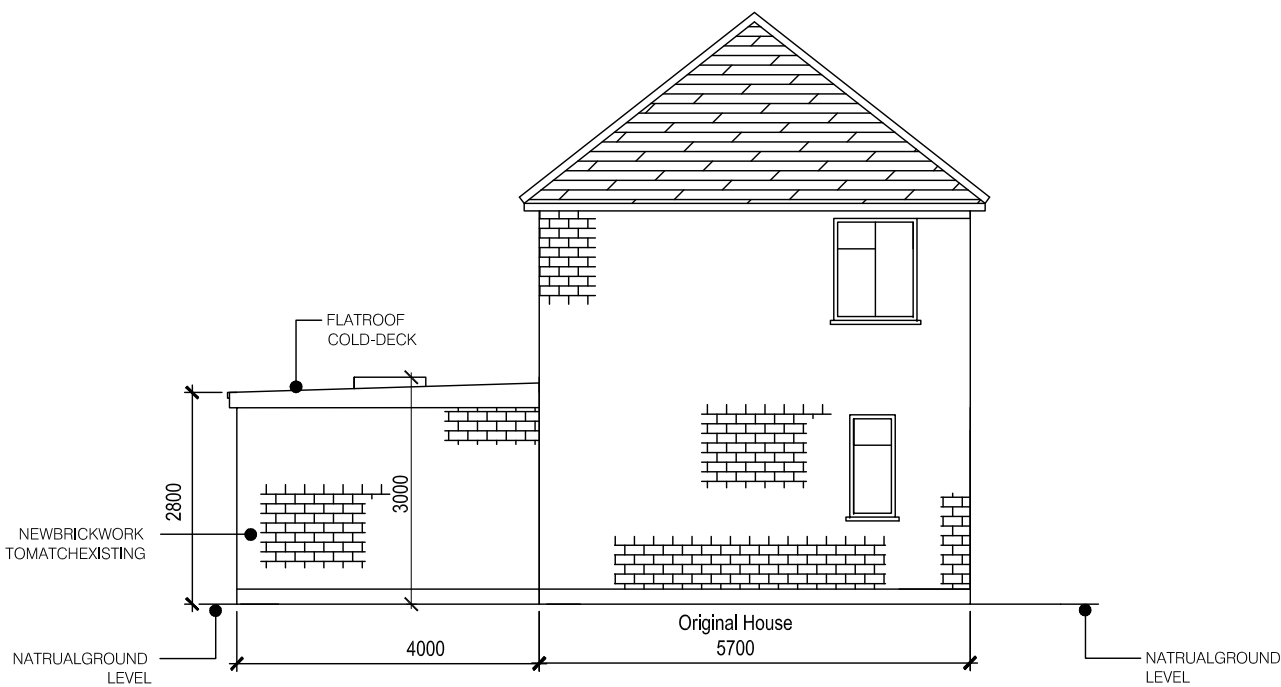
PROPOSED-SIDE ELEVATION (LHSIDE)
