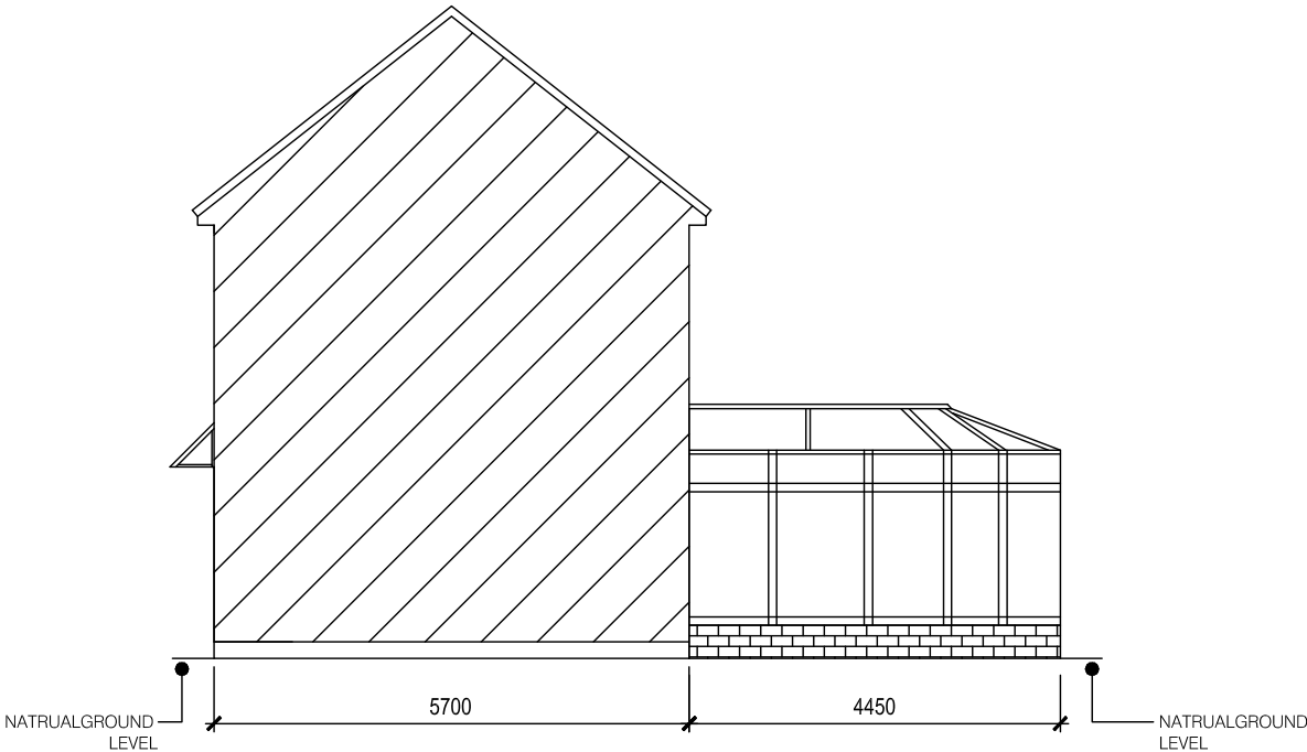
EXISTING-SIDE ELEVATION (RH SIDE)
