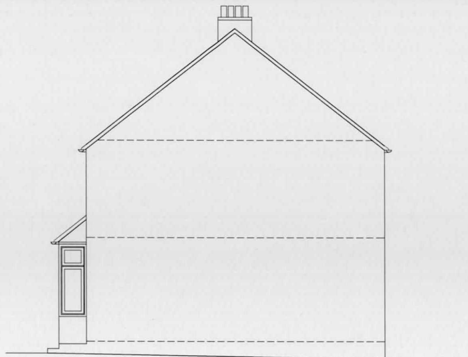
LEFT SIDE ELEVATION (Existing)
