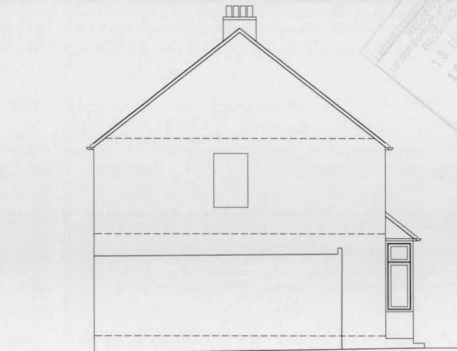
RIGHT SIDE ELEVATION (Existing)
