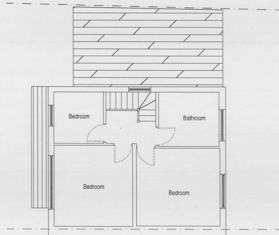
FIRST FLOOR PLAN (Existing)
