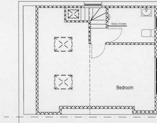
LOFT PLAN (Proposed)
