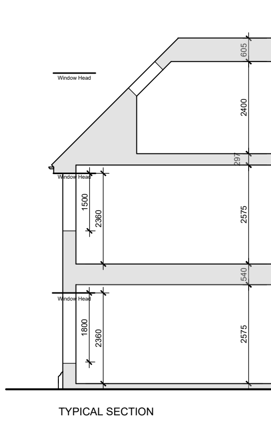
TYPICAL SECTION
