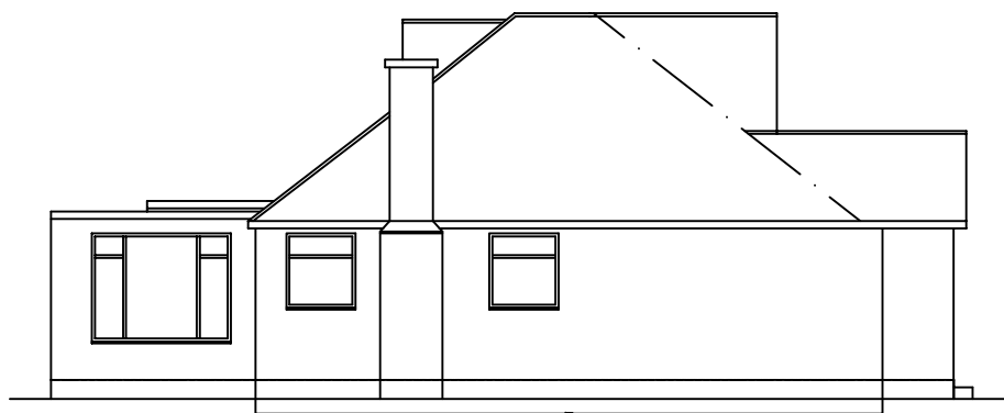
SIDE ELEVATION
