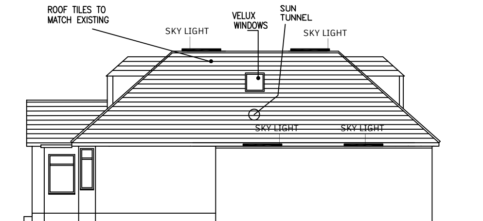
SIDE ELEVATION
