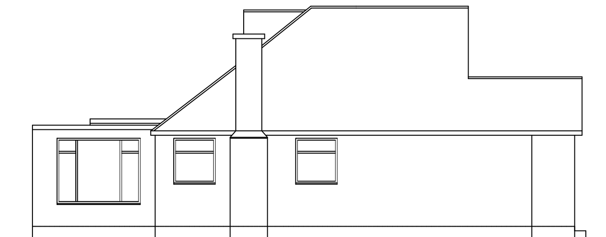
SIDE ELEVATION
