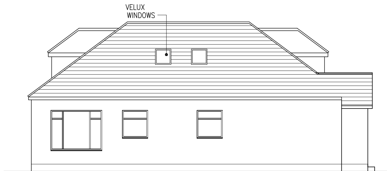
SIDE ELEVATION
