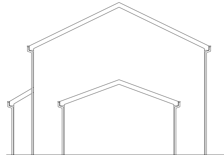
RIGHTSIDE ELEVATION EXISTING
