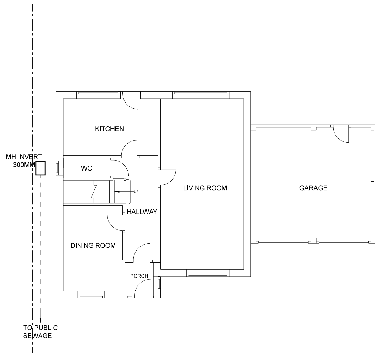
GROUND FLOOR PLAN EXISTING
