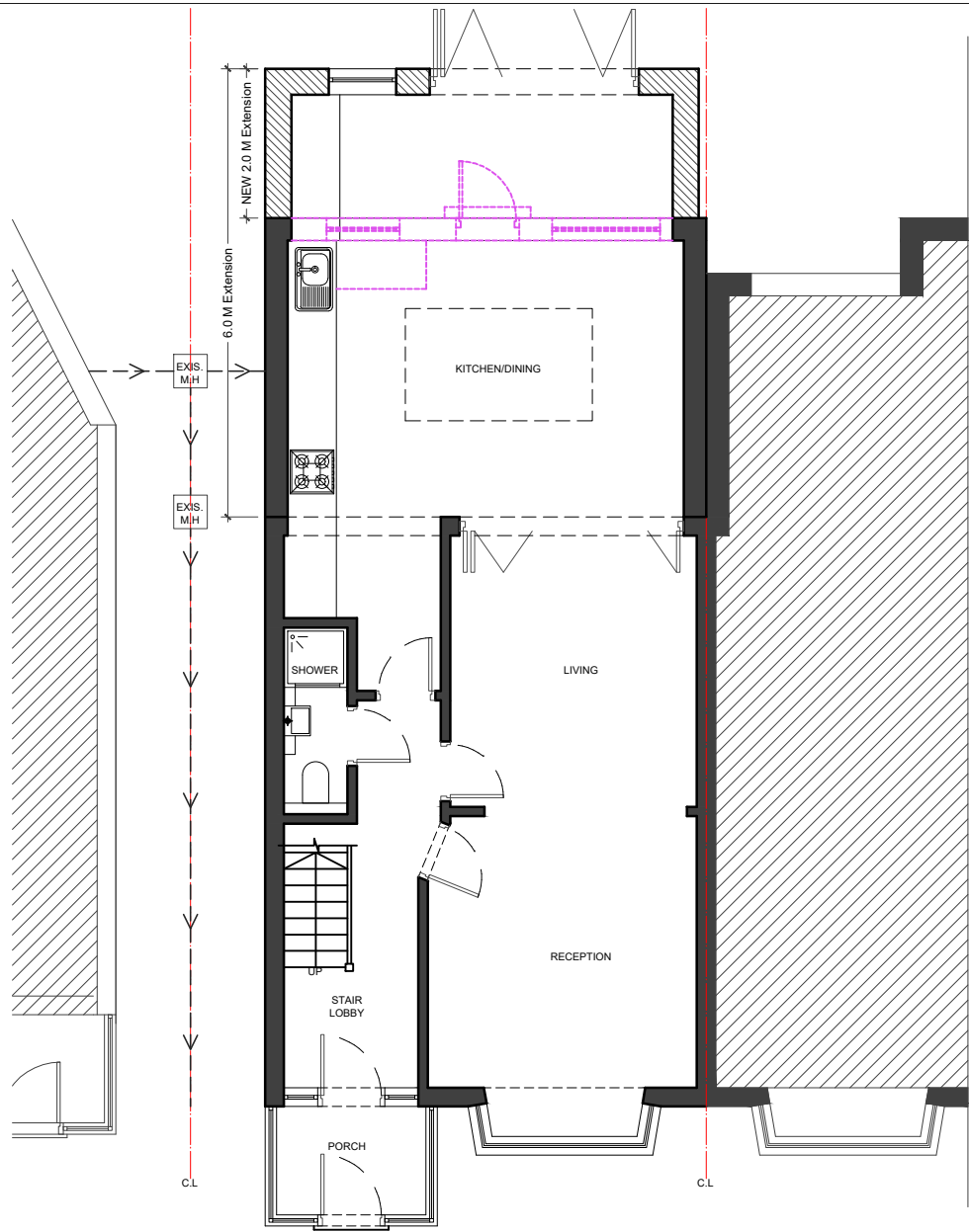
01 - GROUND FLOOR PLAN
