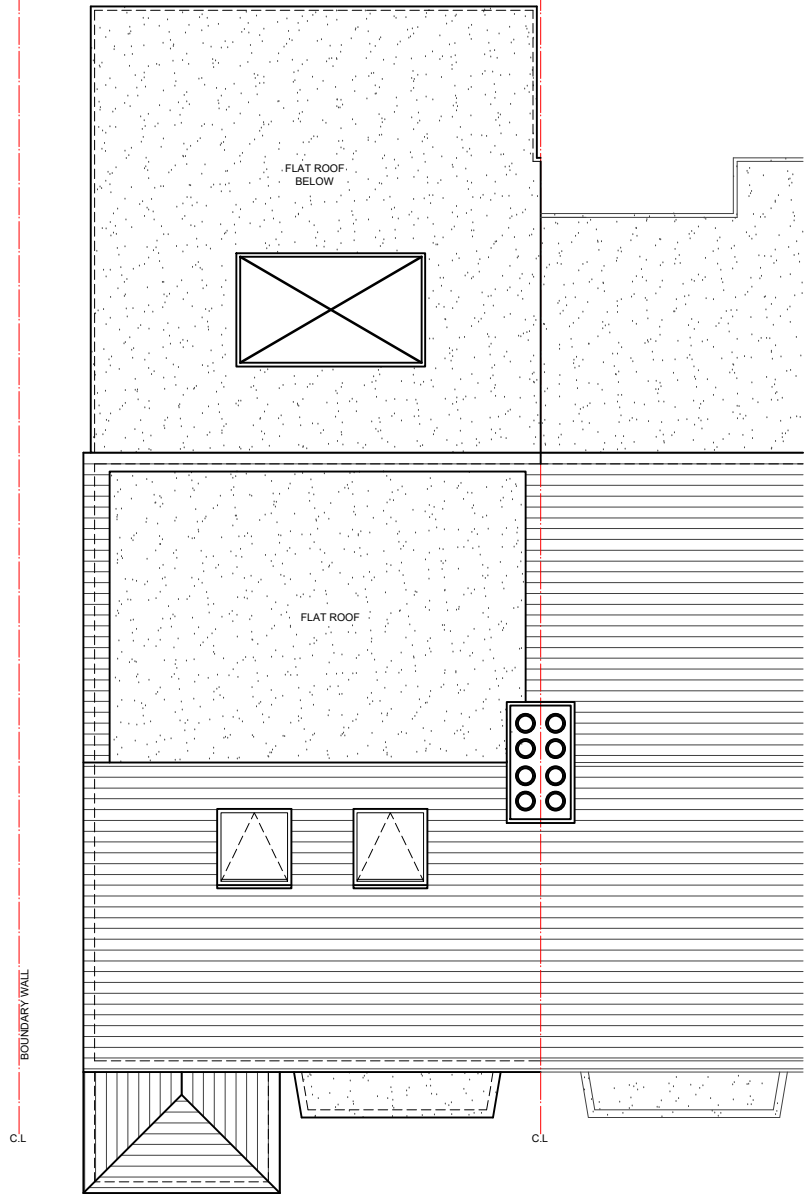
02 - ROOF PLAN
