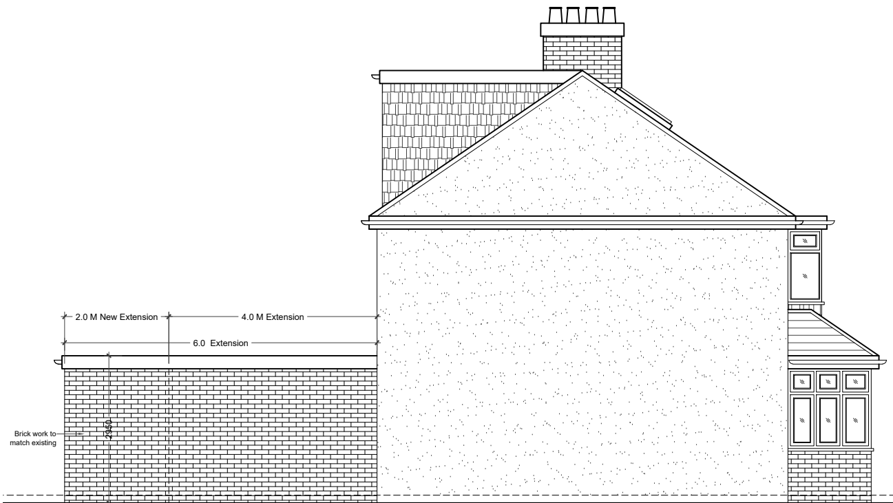
04 - SIDE ELEVATION
