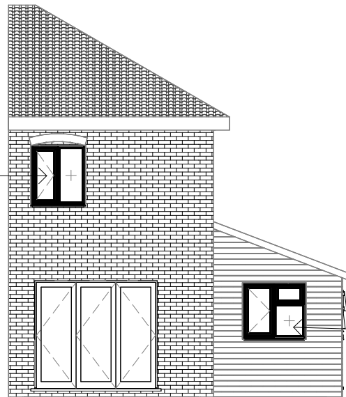
6 Rear Proposed 1 : 100
