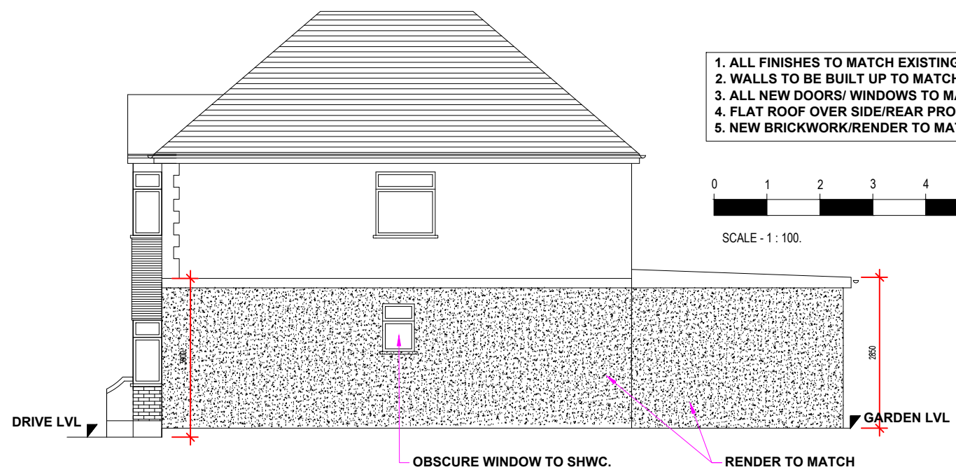
PROPOSED RIGHT ELEVATION
