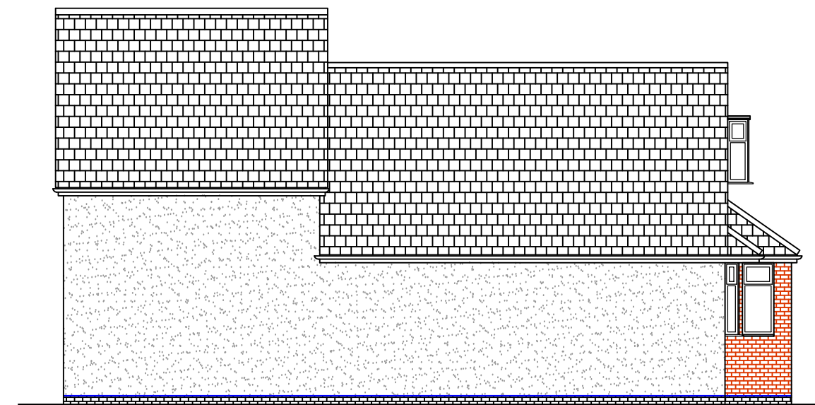
Existing RH Side Elevation
