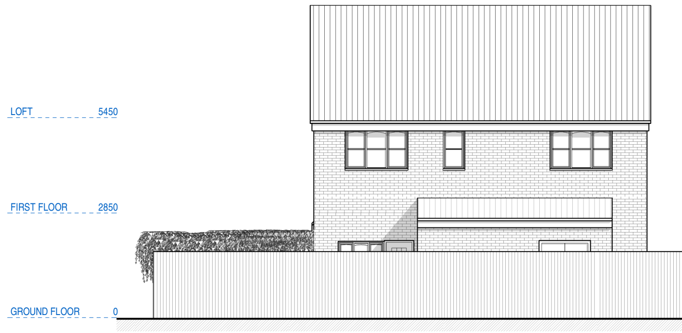
REAR ELEVATION
