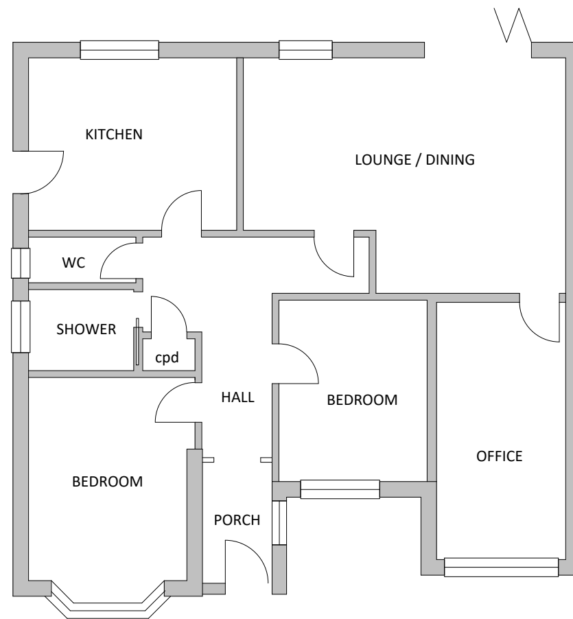
GROUND FLOOR - EXISTING
