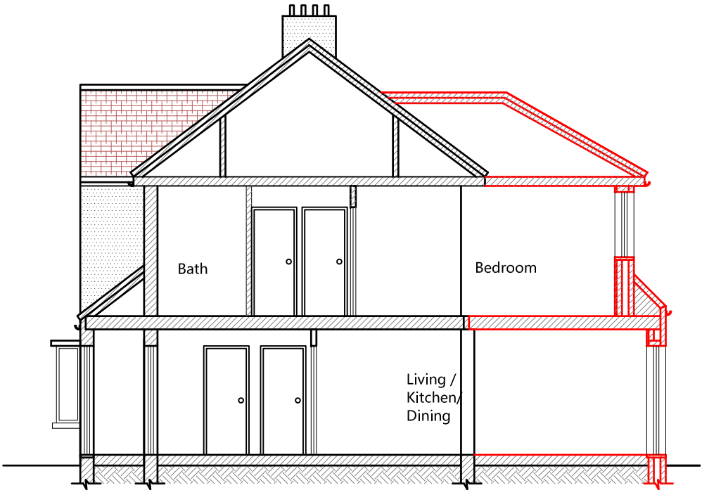
Proposed Section x-x
