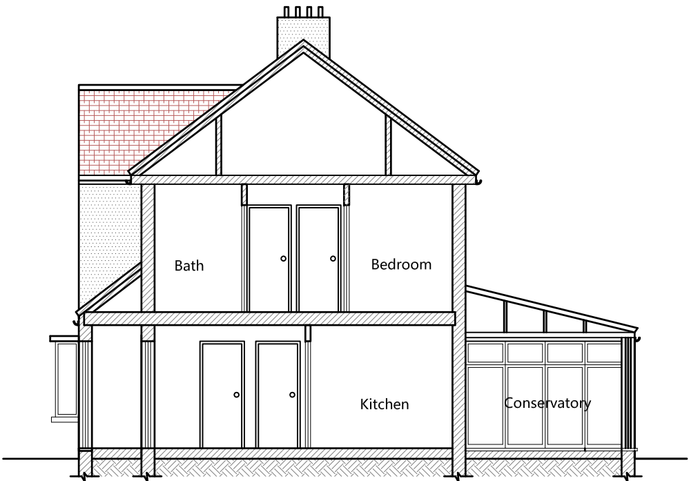
Existing Section x-x
