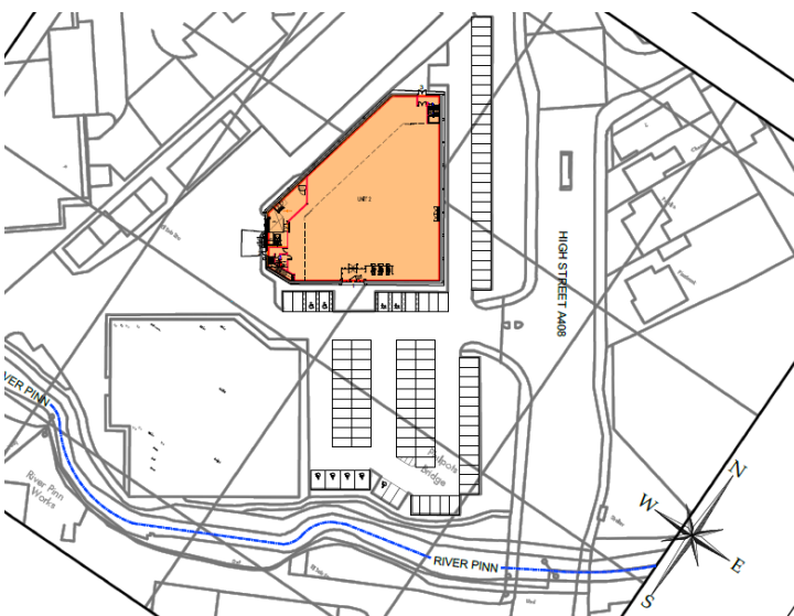
Location Plan
