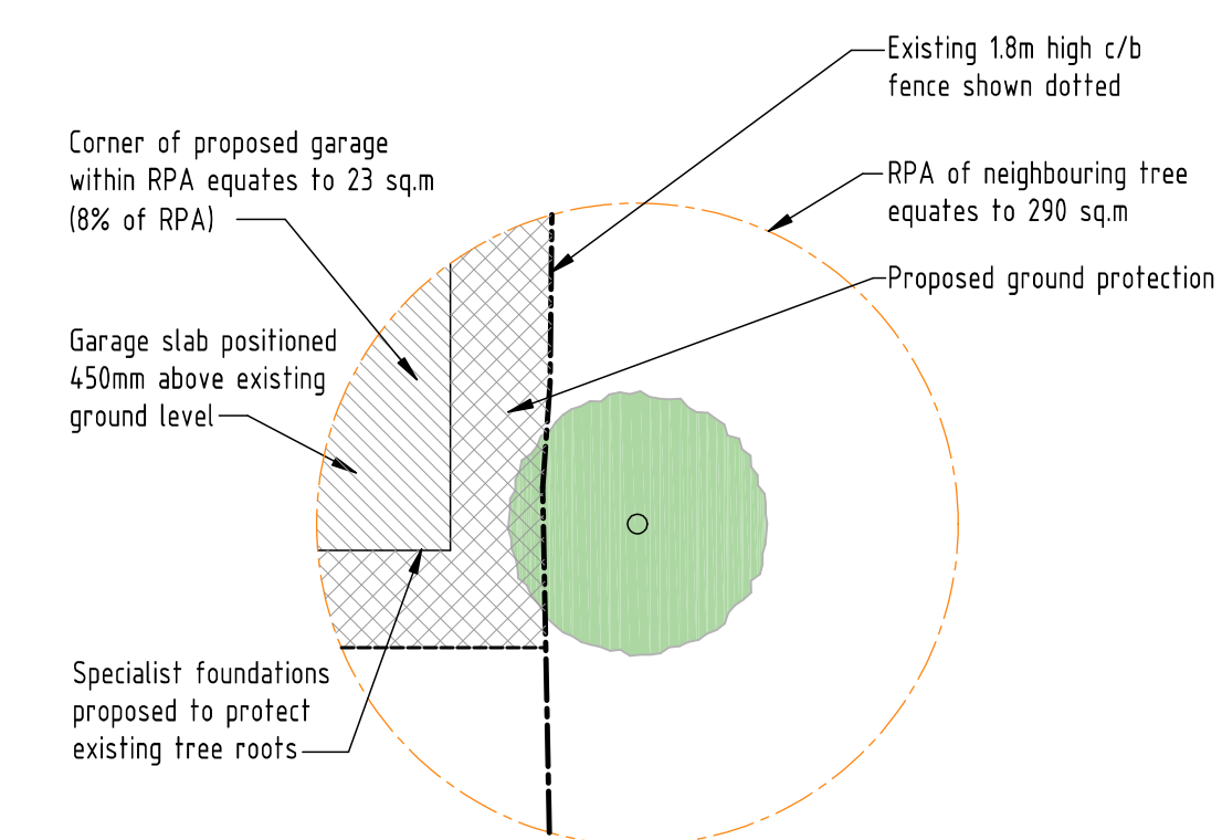
RPA DETAIL - SCALE 1:250
