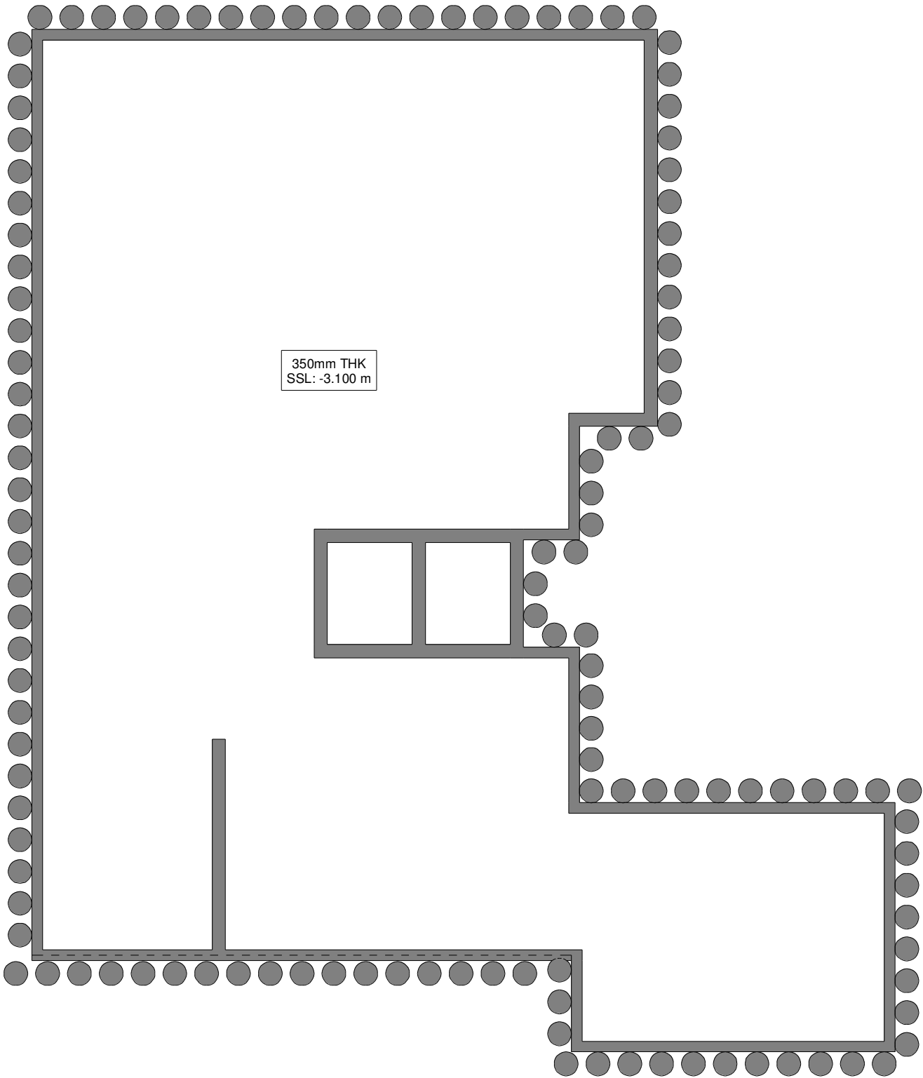
BASEMNT LAYOUT SCALE 1 : 50
