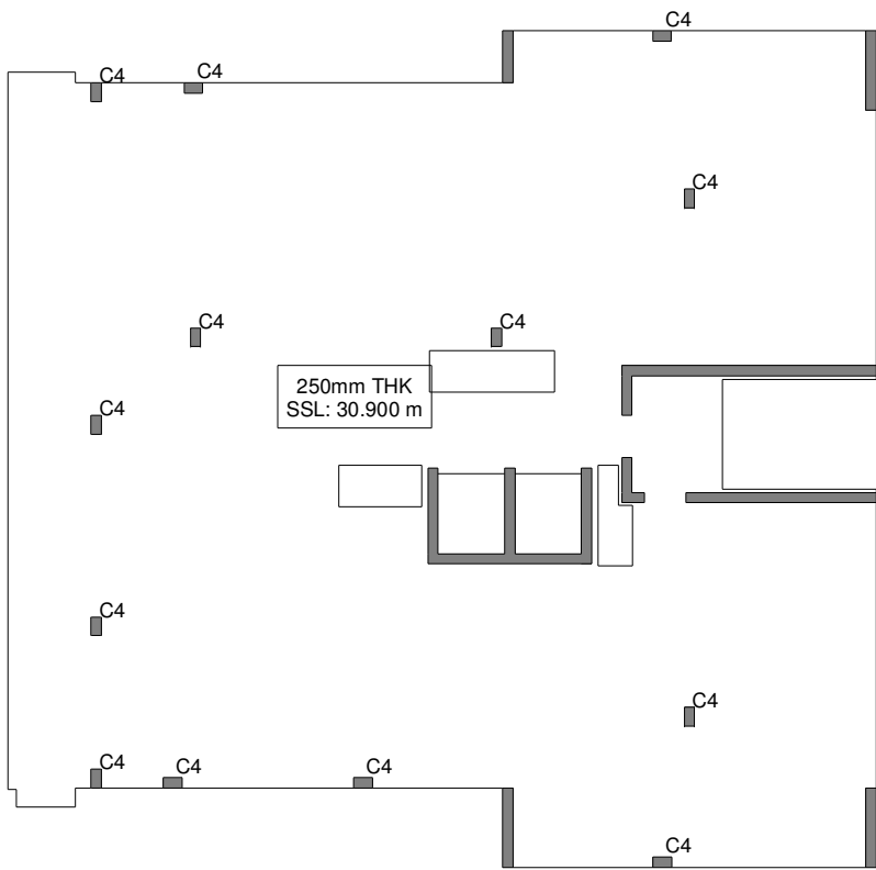
TENTH FLOOR LAYOUT
