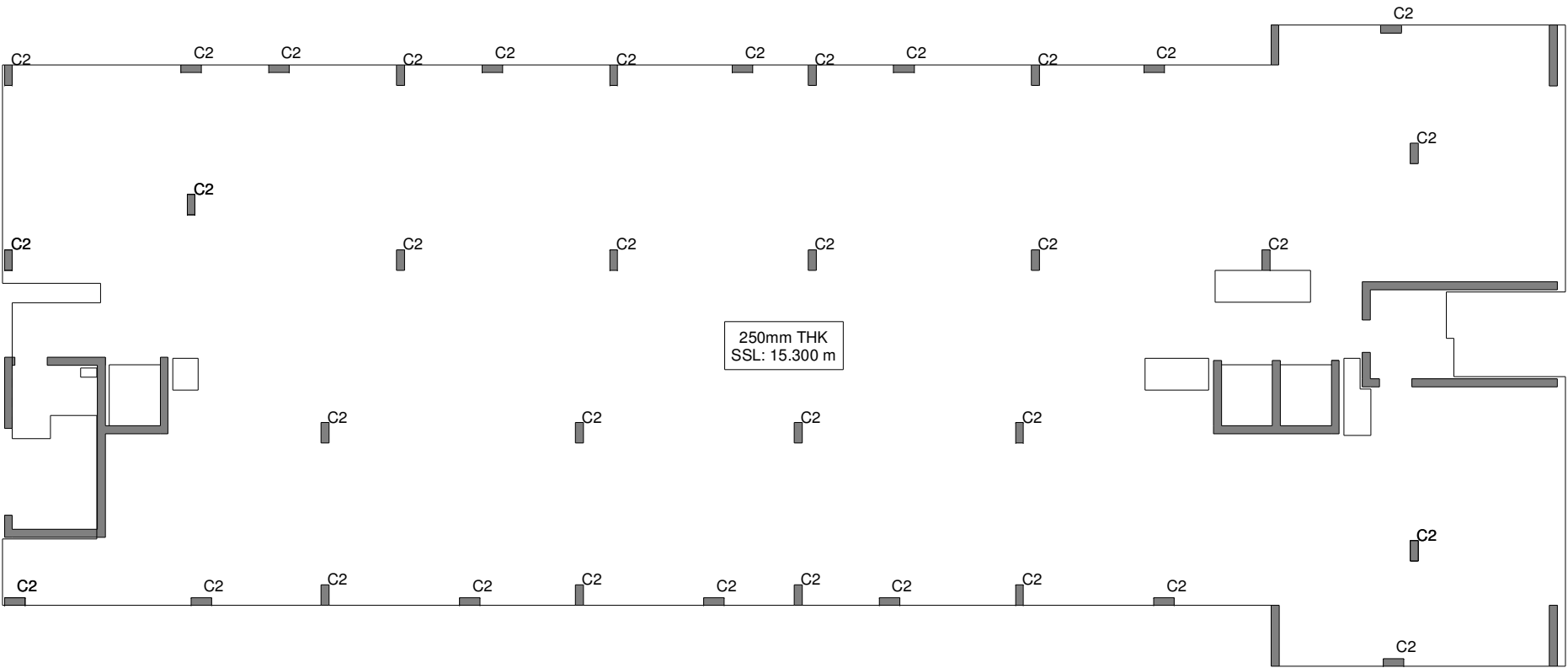
FOURTH FLOOR LAYOUT SCALE 1 : 100
