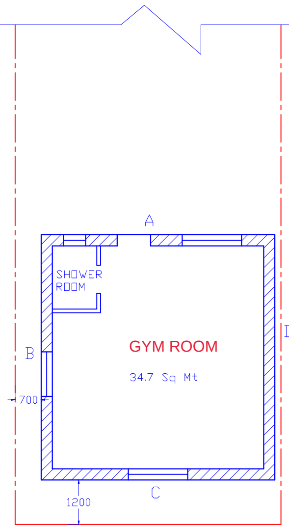
FLOOR PLAN
