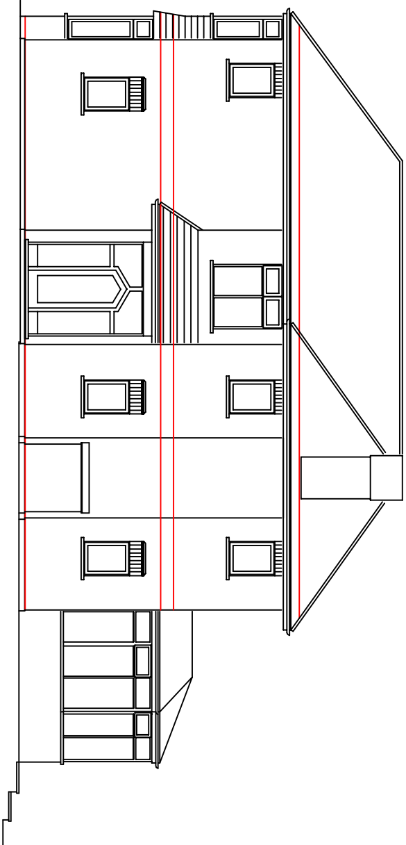
Barnhill (side) elevation
