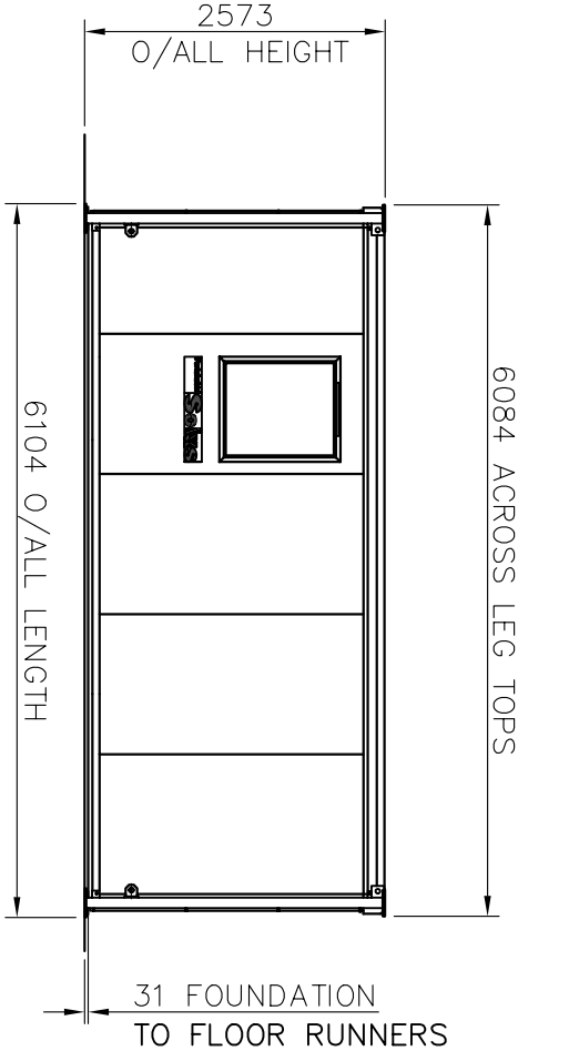
REAR ELEVATION
