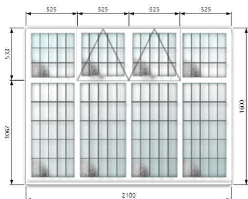
Front 1st Old w6
