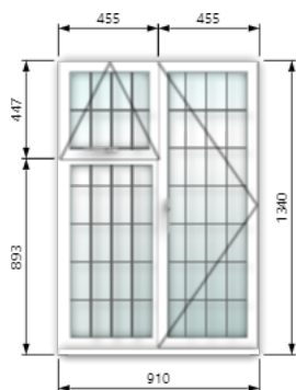
side elevation W2
