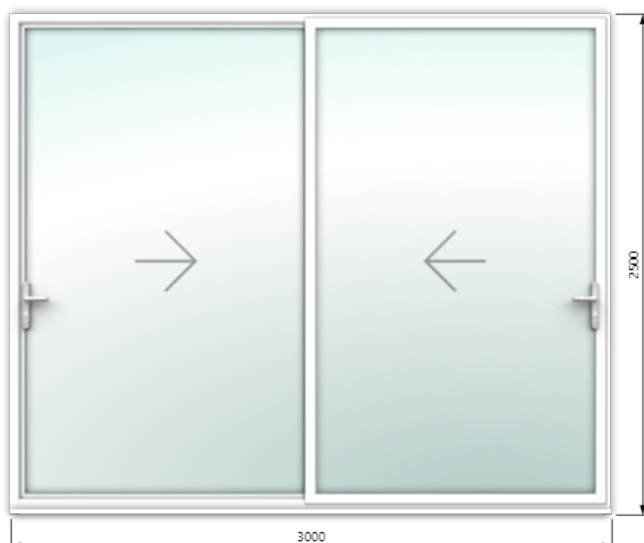
side elevation Slim slider D4
