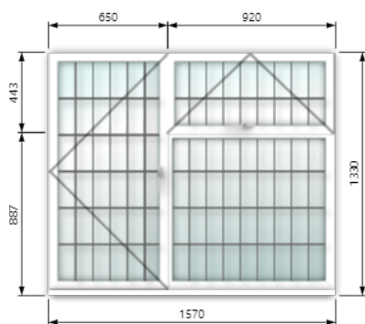
Side elevation
