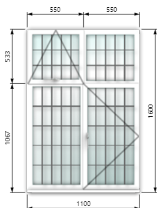
Front 1st Old w5
