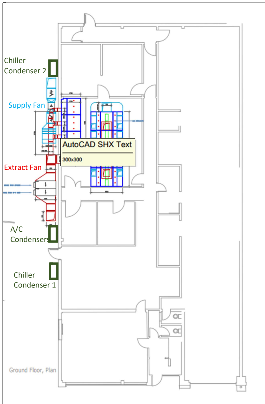
Figure 5.1 Location of supply / extract fans and Chillers (Image Source: Nationwide Ventilation)
