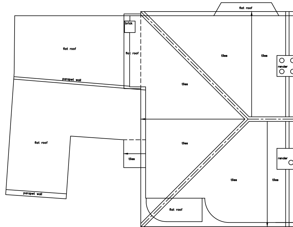
ROOF PLAN EXISTING
