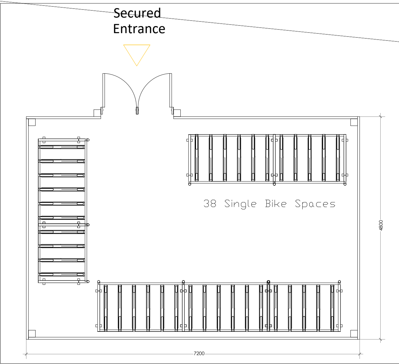
PLAN OF SECURE CYCLE PARKING
