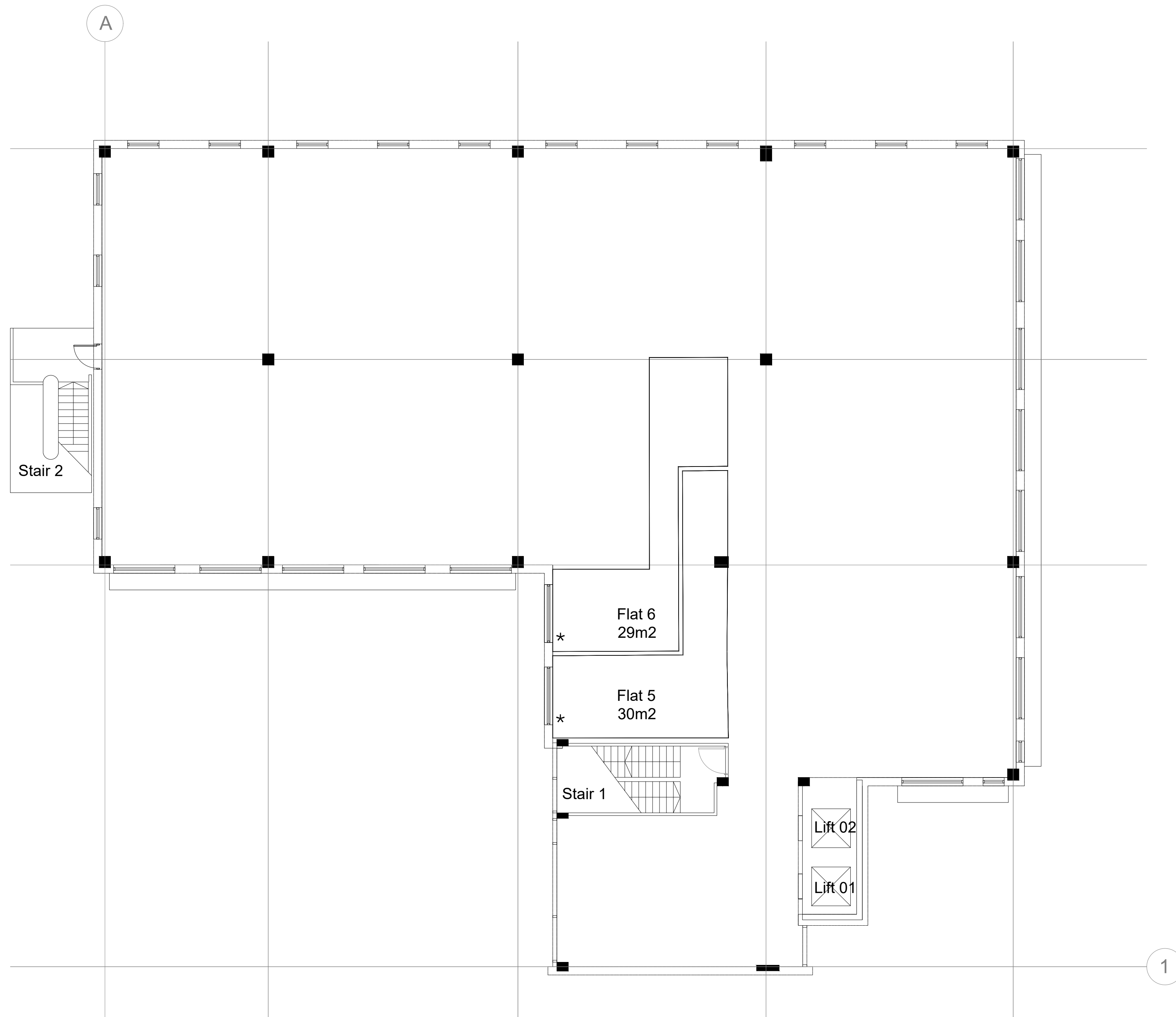
Proposed Second Floor Plan
