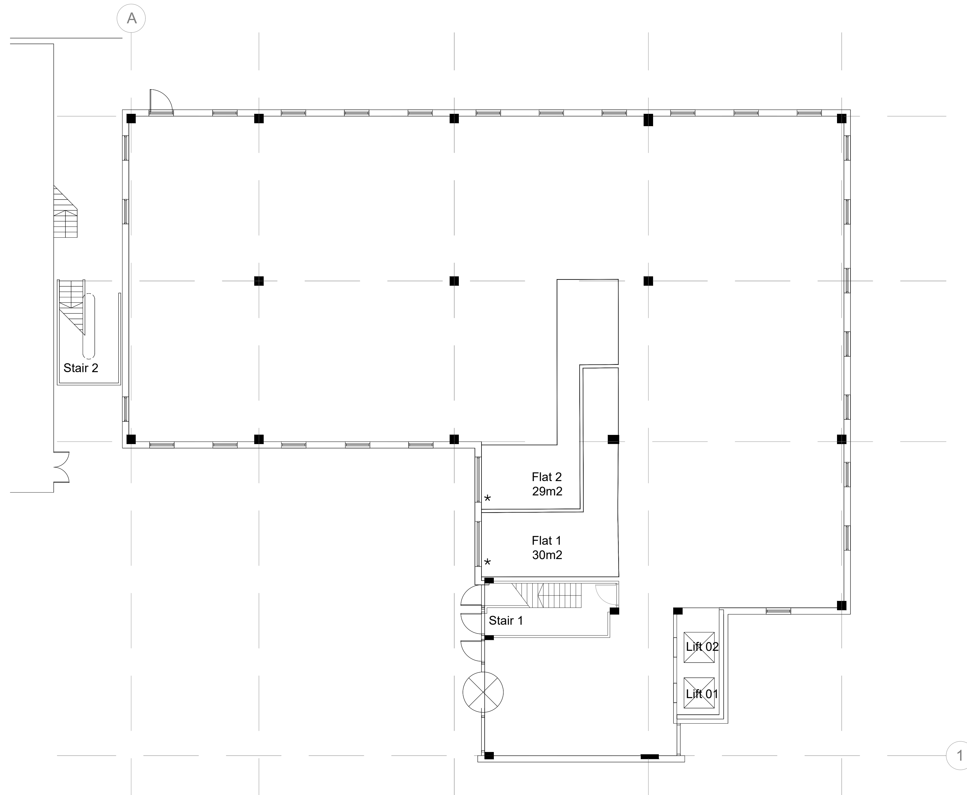
Proposed Ground Floor Plan * new aluminium windows to match existing as part of separate application
