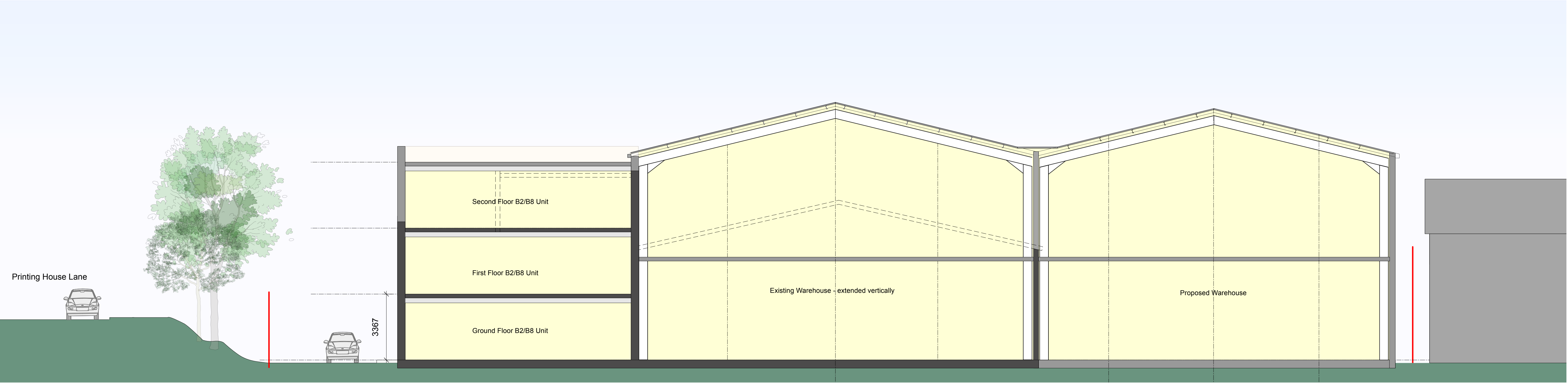
2 Proposed Section A-A Scale: 1:100
