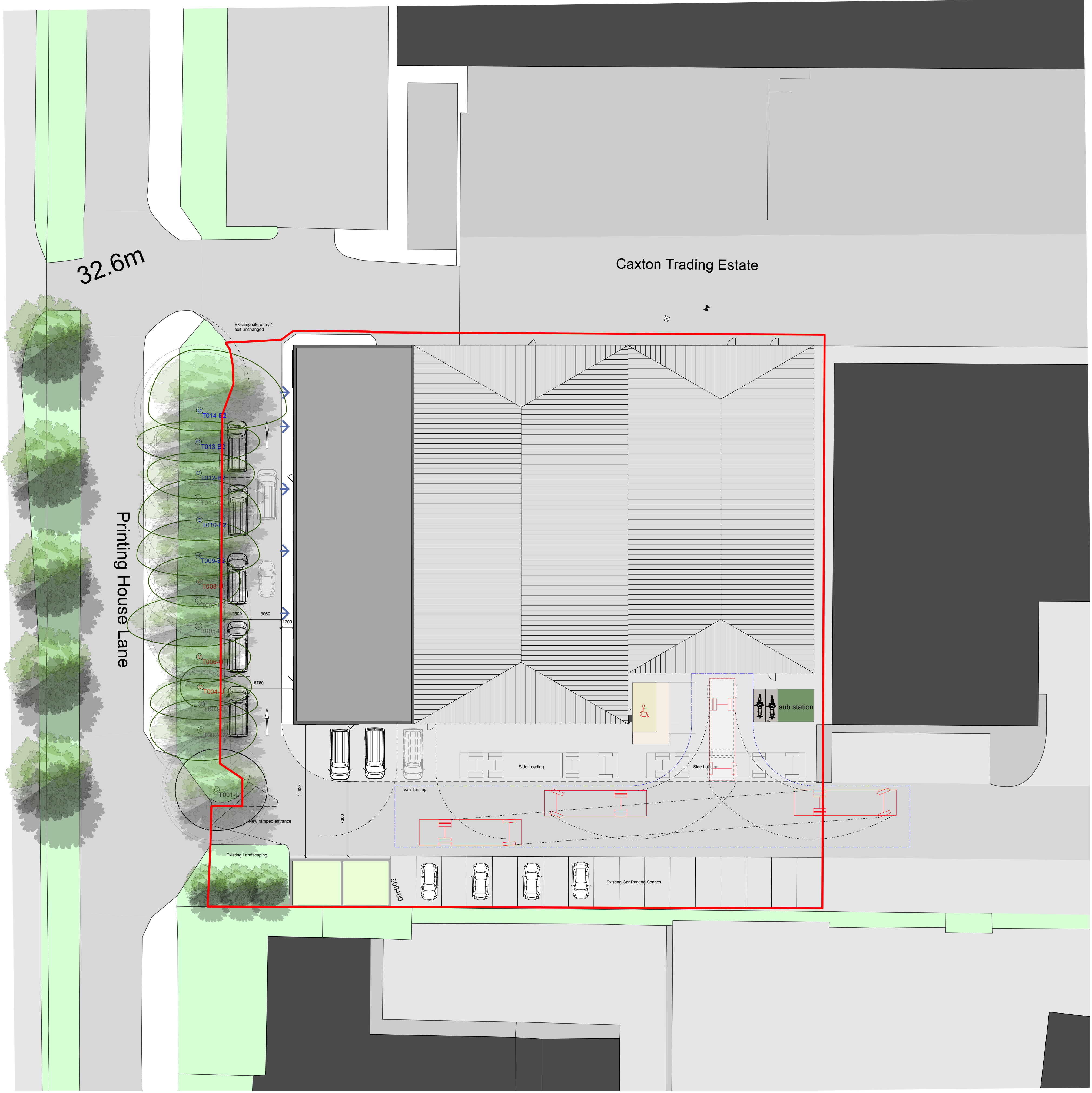
Proposed Block Plan Scale: 1:200
