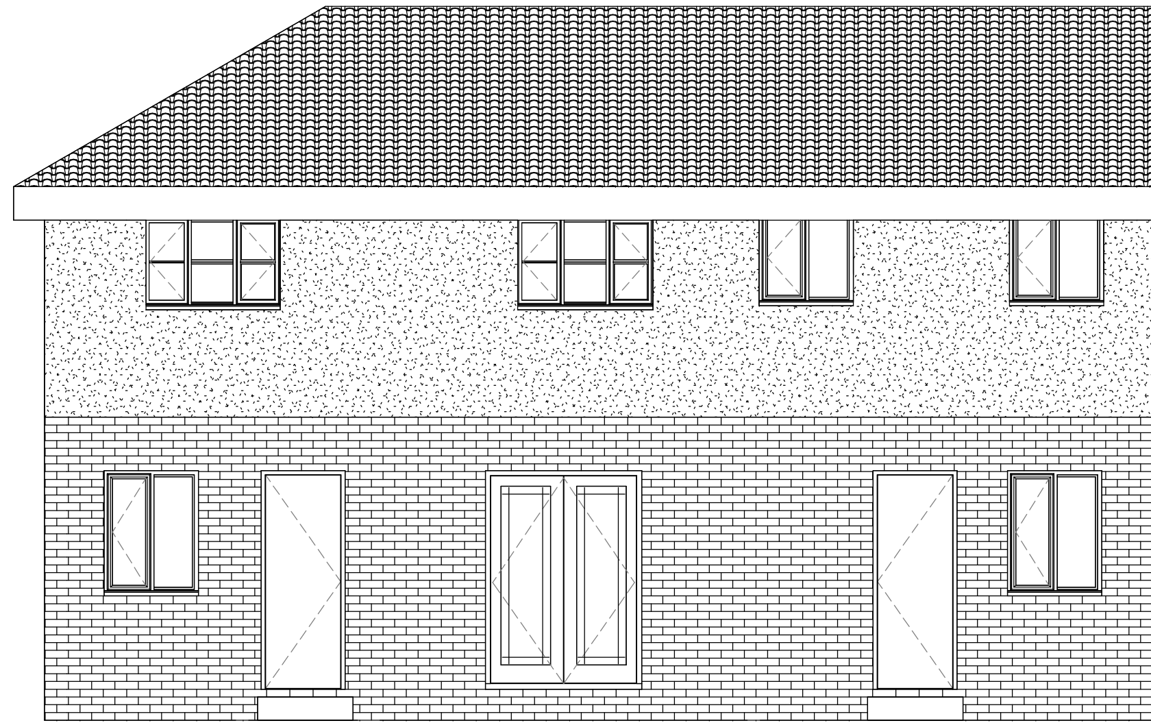
1 EXISTING REAR ELEVATION 1 : 50
