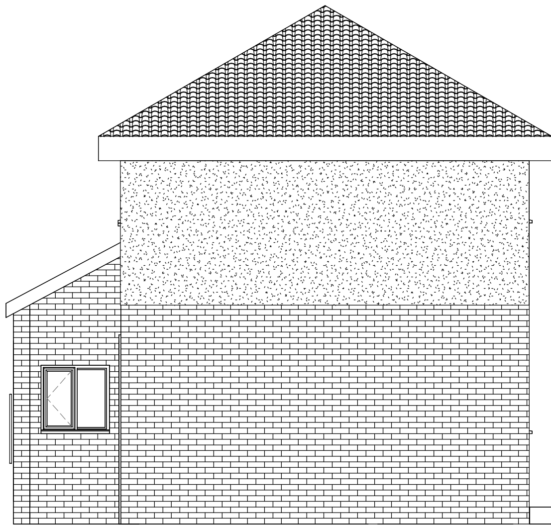
2 EXISTING SIDE ELEVATION 1 : 50
