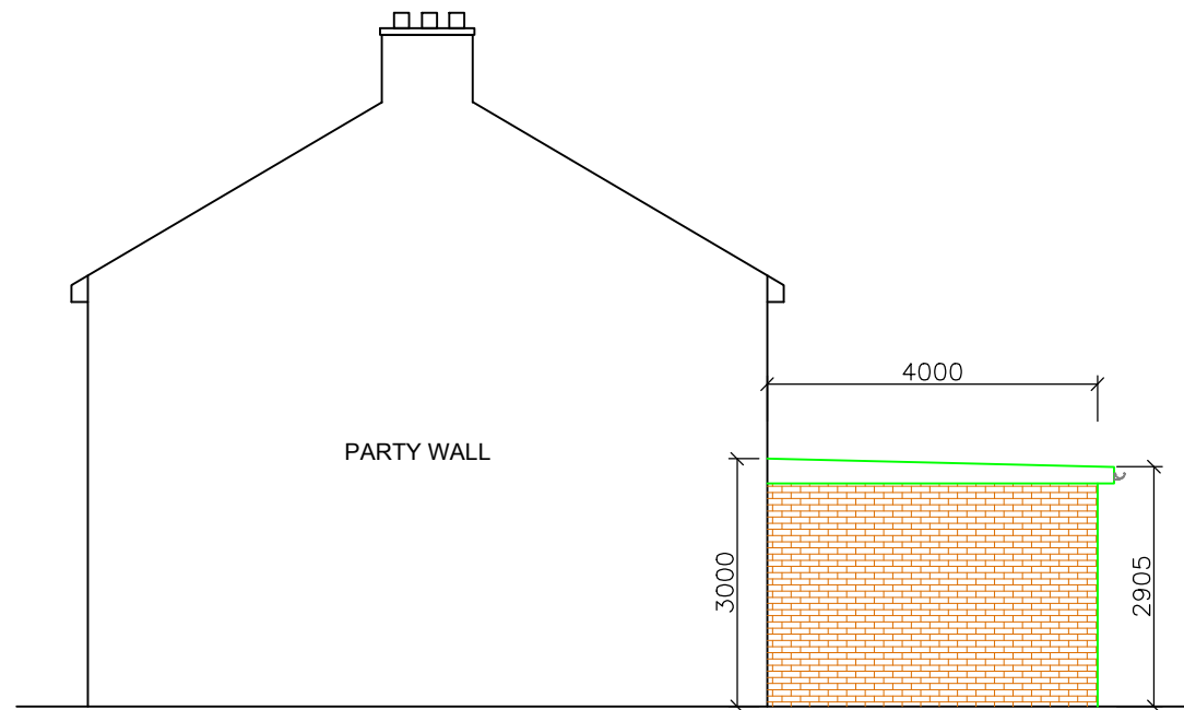
PROPOSED SIDE ELEVATION(P#106) SCALE= 1:100
