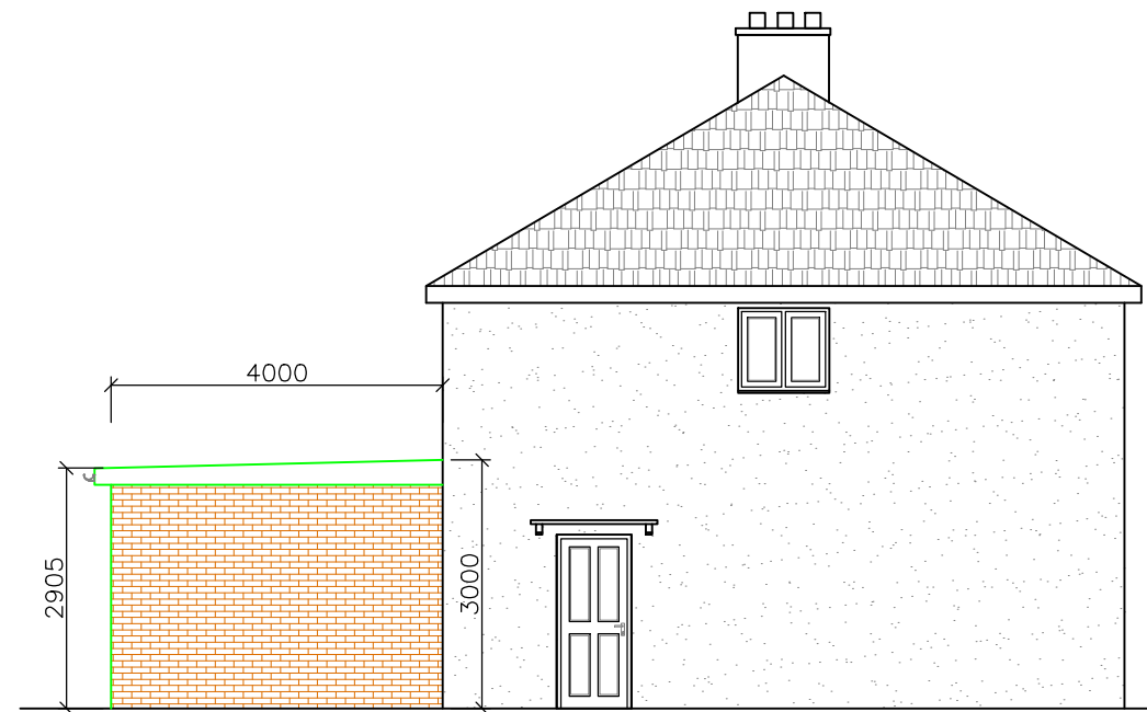
PROPOSED SIDE ELEVATION (P#104A) SCALE= 1:100
