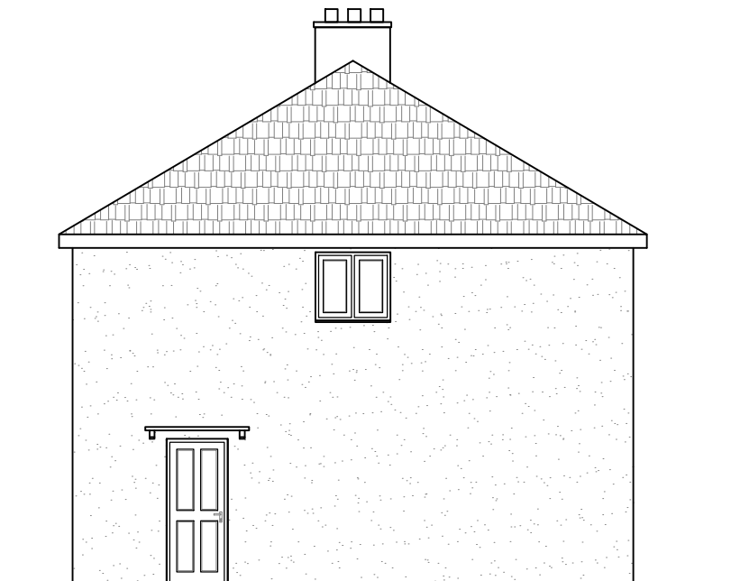
EXISTING SIDE ELEVATION (P#104A) SCALE= 1:100
