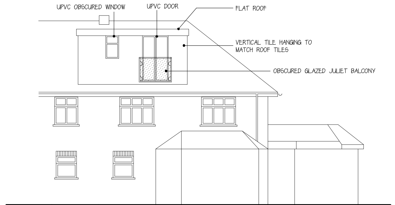
REAR ELEVATION
