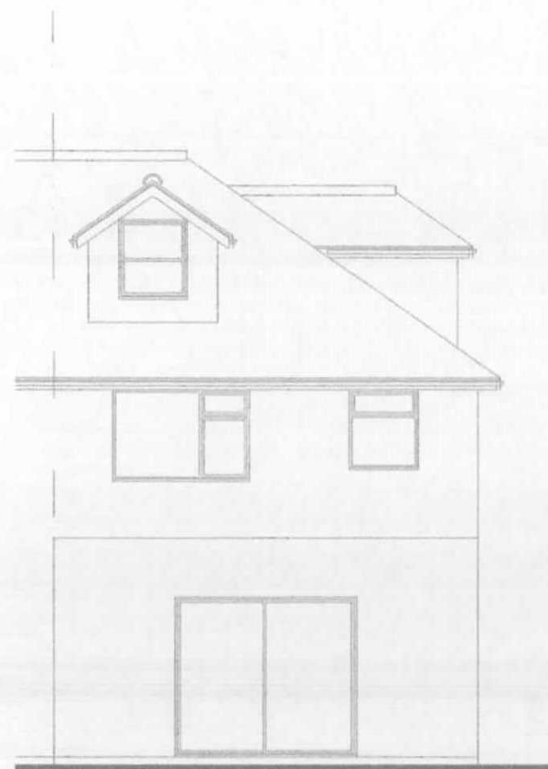
SOUTH ELEVATION.
