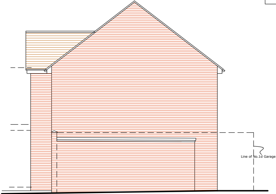
WEST ELEVATION
