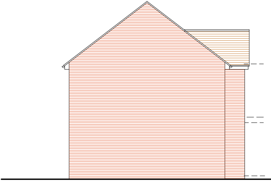
EAST ELEVATION
