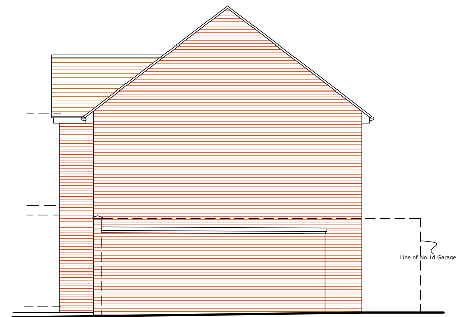
WEST ELEVATION
