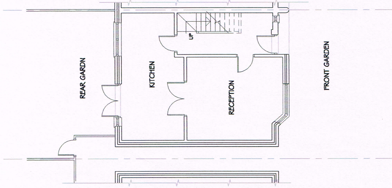
EXISTING GROUND F. PLAN SCALE 1 : 100
