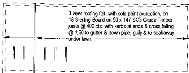
Roof Plan
