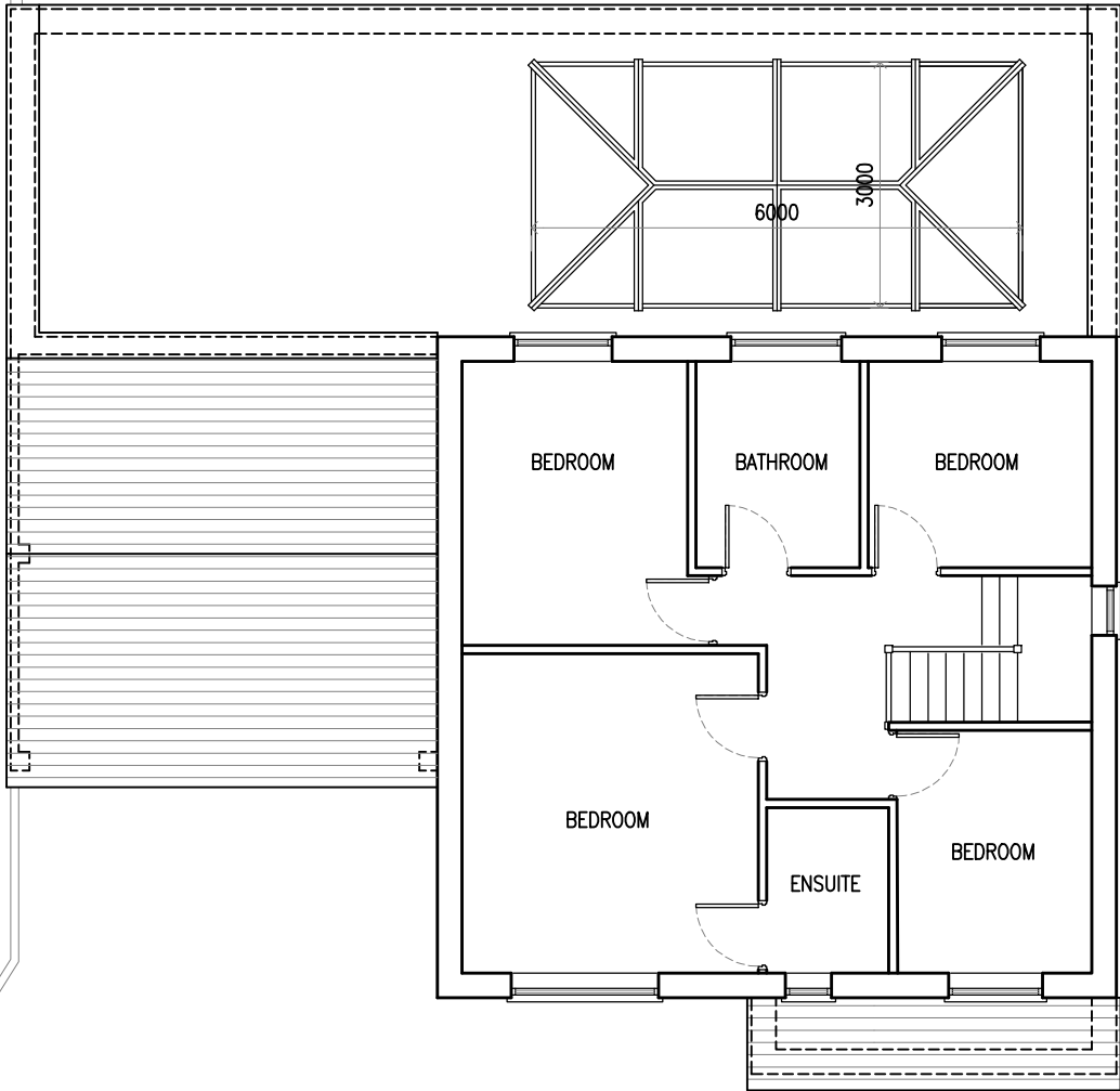
FIRST FLOOR
