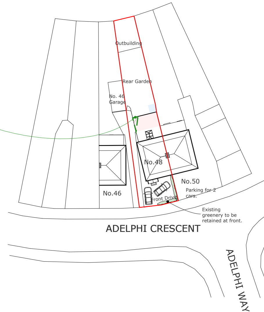
Block Plan
