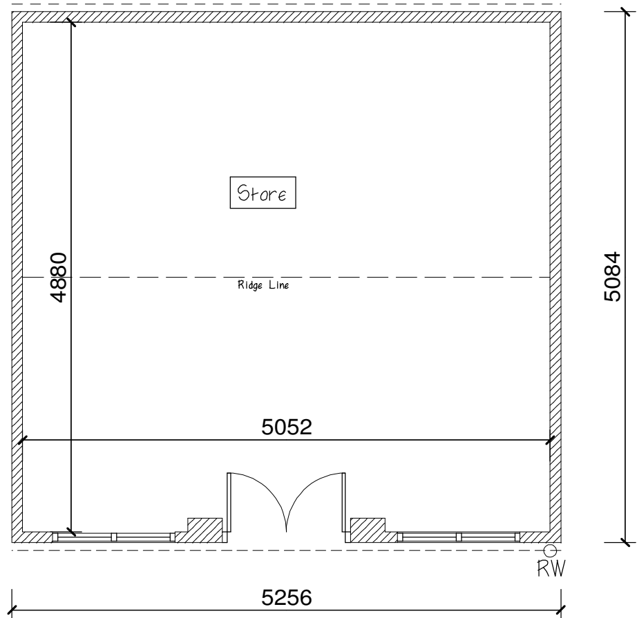
Floor plan
