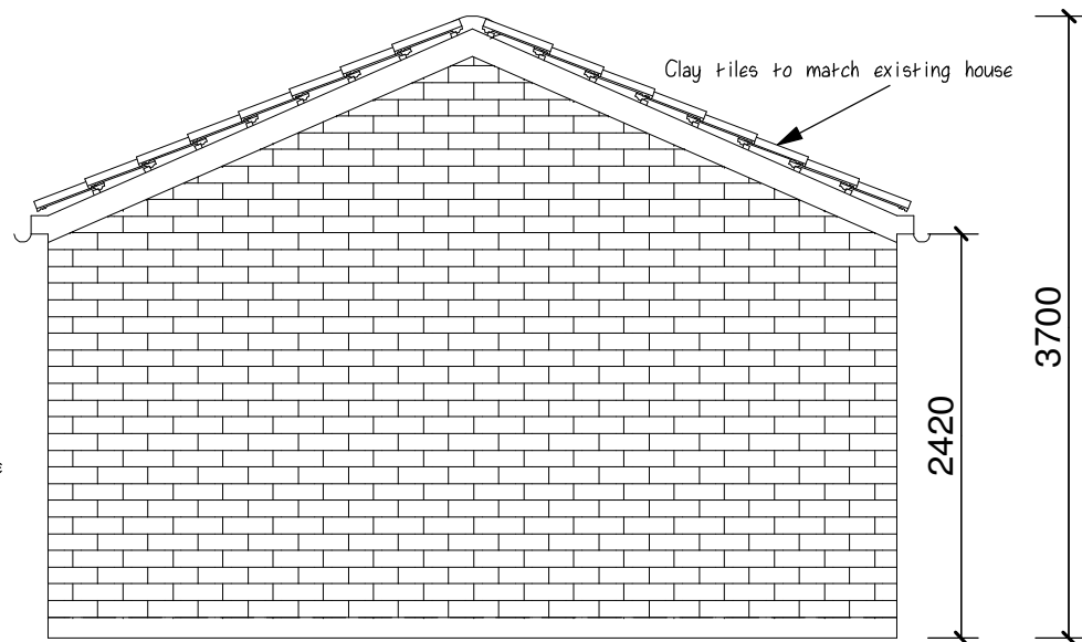
Side Elevation Adjacent #87
