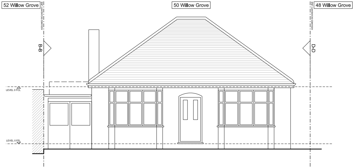
3. EXISTING FRONT ELEVATION (A-A)
