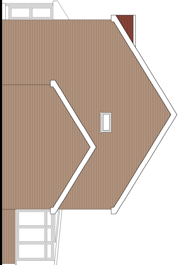
EXISTING RIGHT SIDE ELEVATION 1:100
